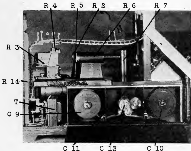
FIG. 3. Photograph of left side of graininess photometer half assembled. (The designations refer to those in Fig. 1.)
